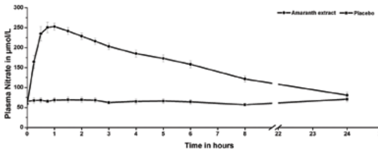
Plasma Nitrate (NO 3 - ) level after administration of Oxystorm® and placebo
